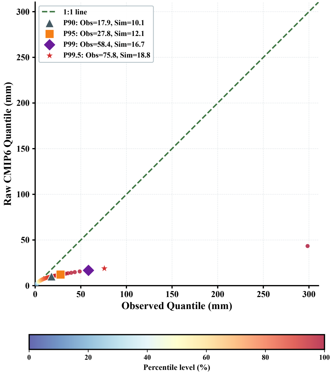
(a) Observed vs Raw CMIP6 QQ-RMSE = 19.47 mm
