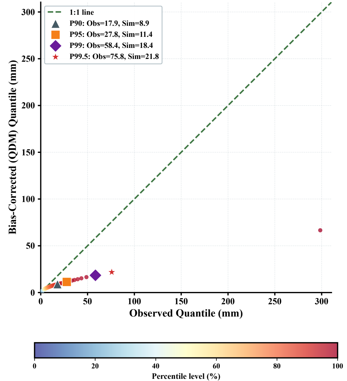
(b) Observed vs BC (QDM) QQ-RMSE = 17.98 mm
